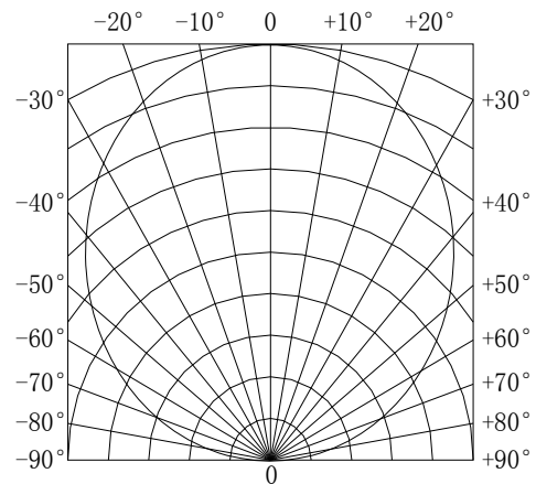
Fig.6 Spatial Distribution
